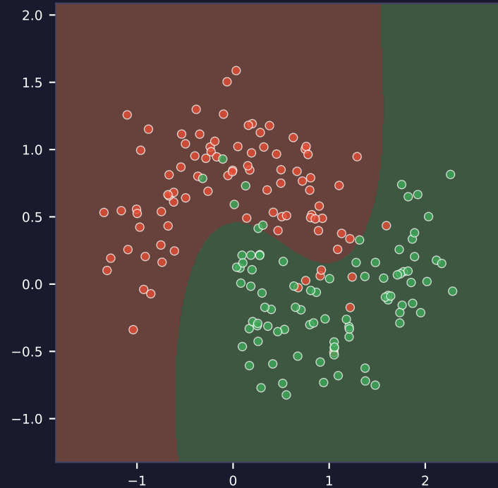
SVM RBF Acc=0.972
