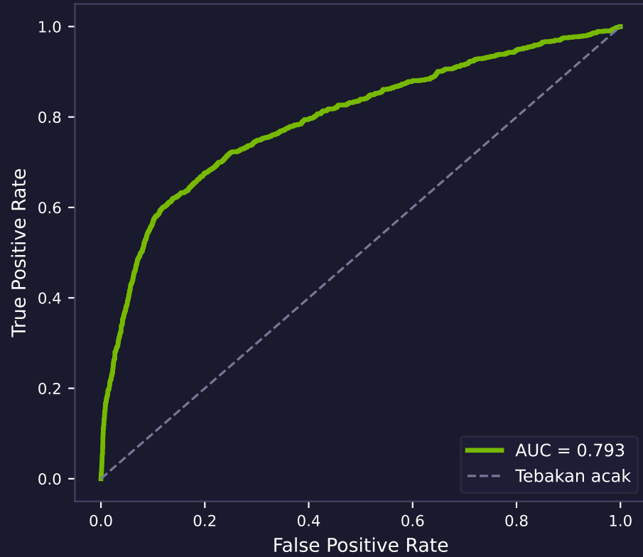
ROC Curve
