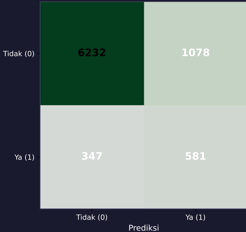
Confusion Matrix
