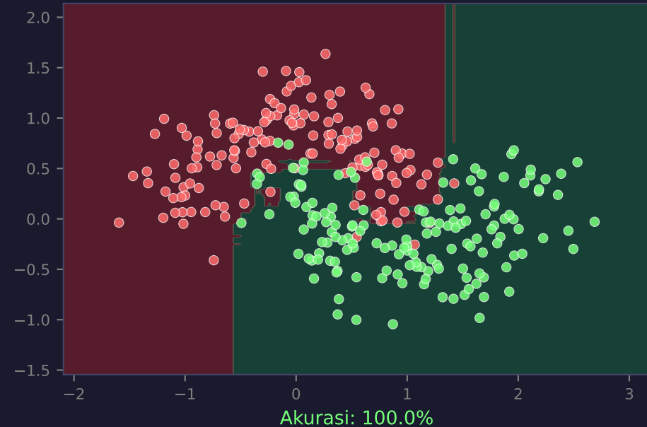
Random Forest (Bagging)
