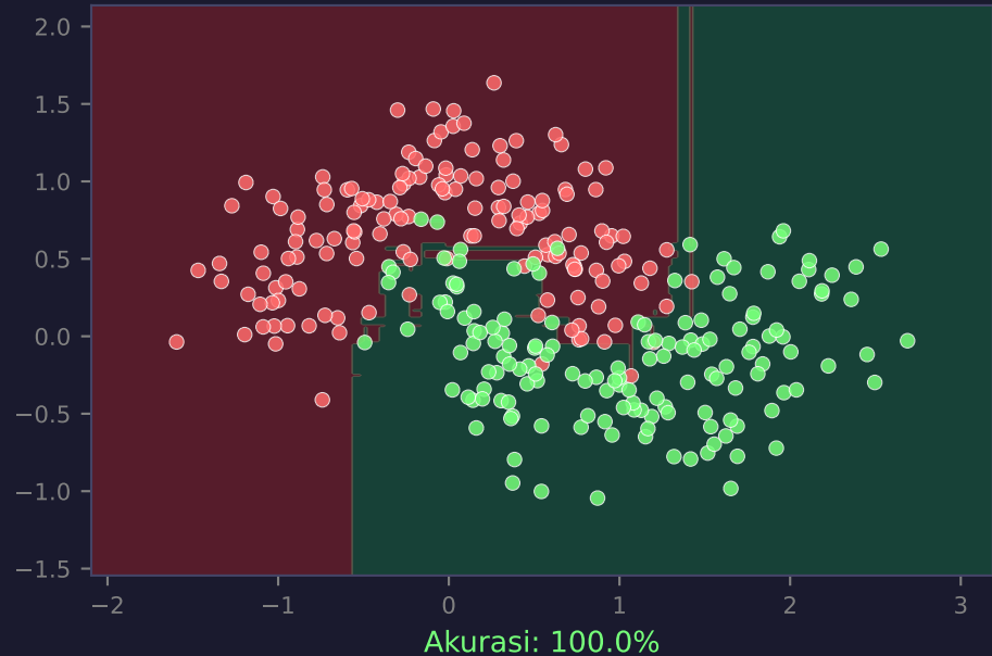
Gradient Boosting
