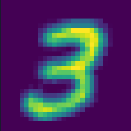
feature map 7
