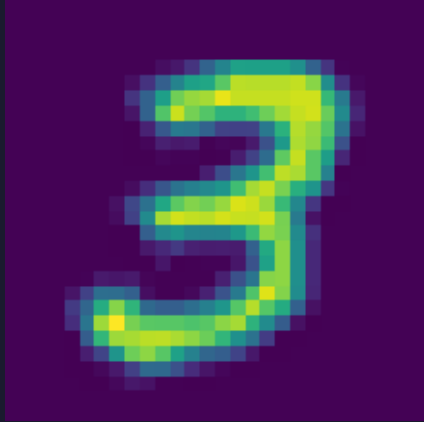
feature map 8
