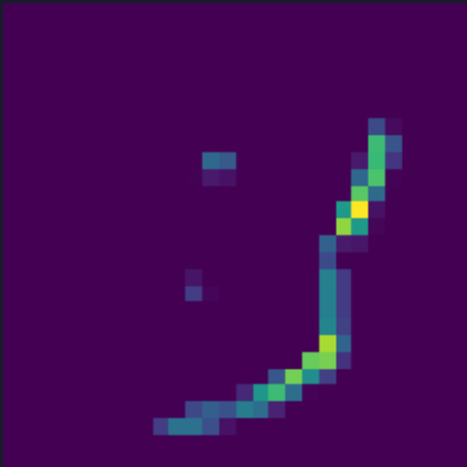
feature map 1
