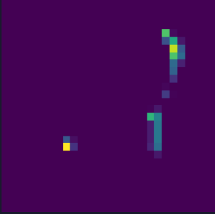
feature map 3
