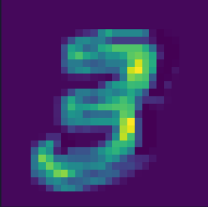
feature map 6
