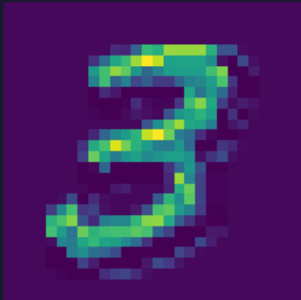
feature map 2
