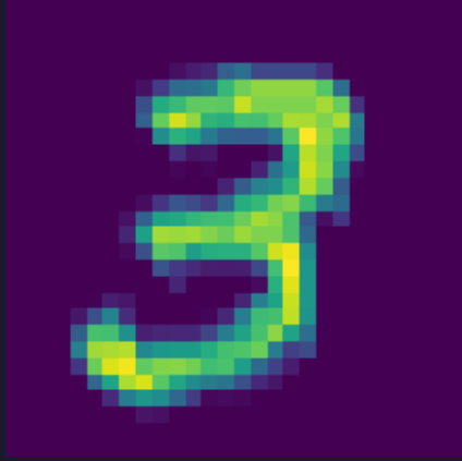
feature map 5
