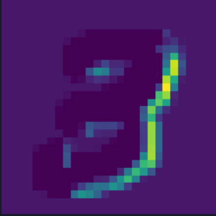
feature map 4
