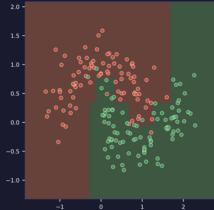
Decision Tree Acc=0.972
