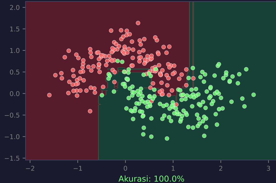
Gradient Boosting
