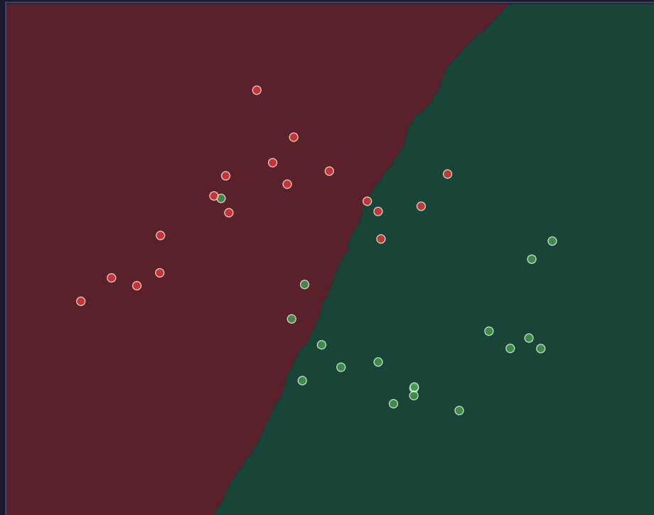
Underfitting
