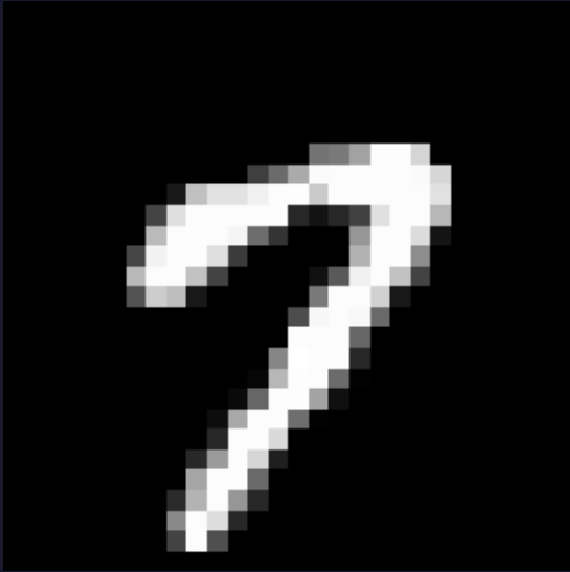
Gambar input (digit 7)
