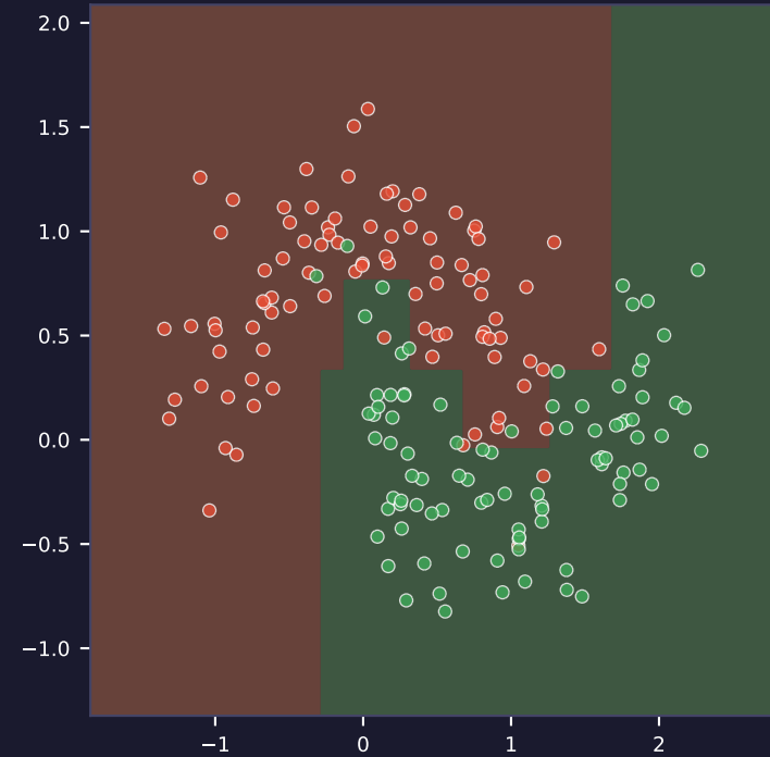
Decision Tree Acc=0.972
