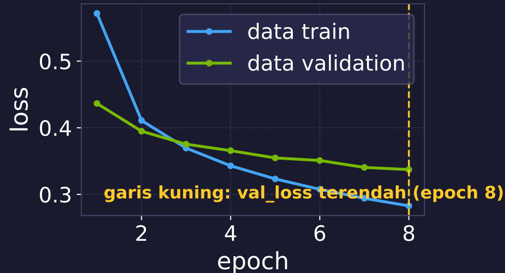
Loss
