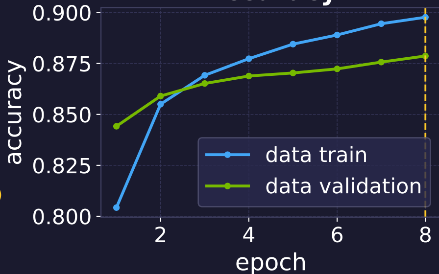
Accuracy
