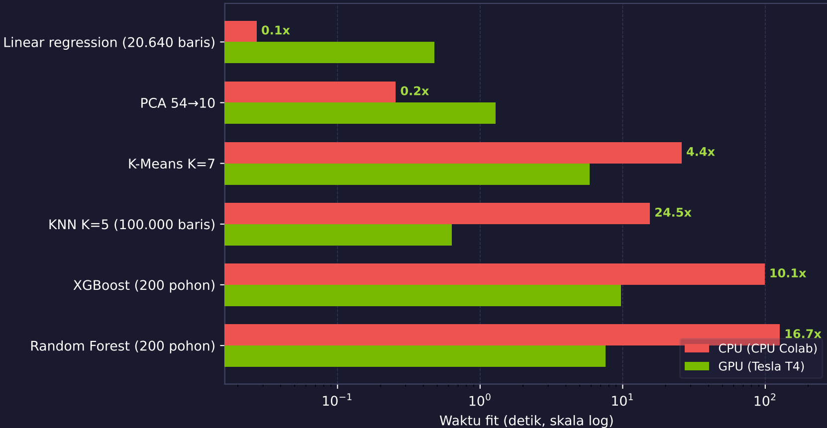
Covertypes, 581.012 baris — Tesla T4 vs CPU Colab
