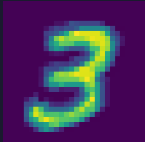
feature map 8
