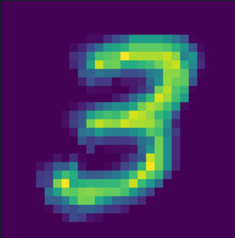
feature map 7
