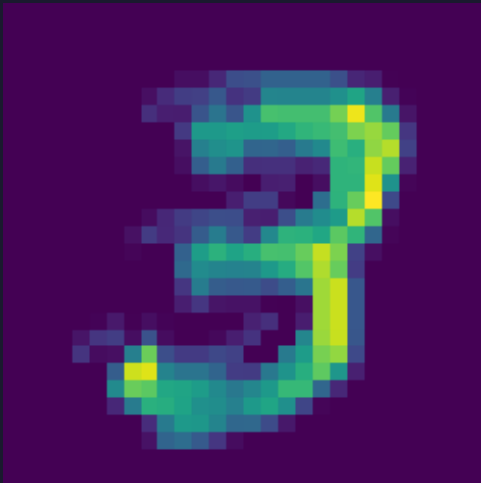
feature map 6
