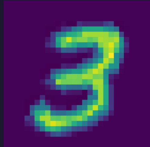
feature map 5
