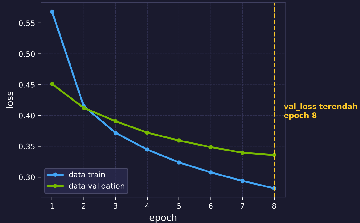
Loss
