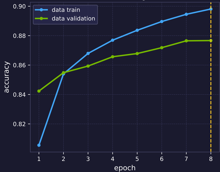
Accuracy
