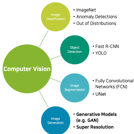
Image Generation
