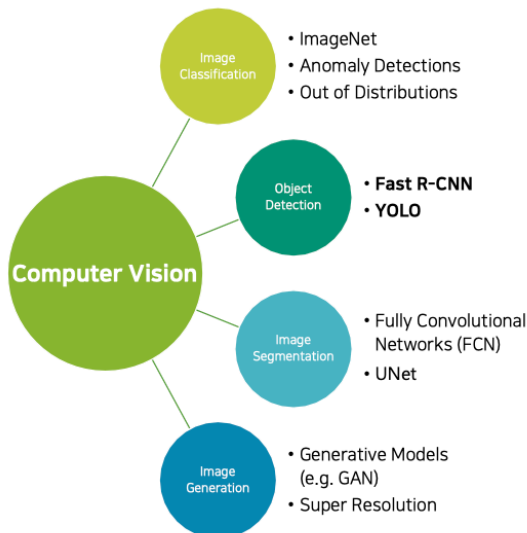
Object Detection
