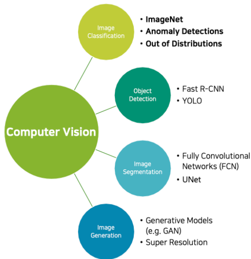
Image Classification
