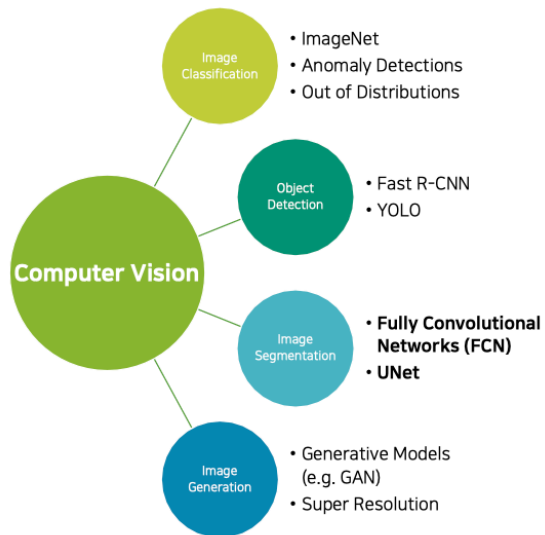
Image Segmentation
