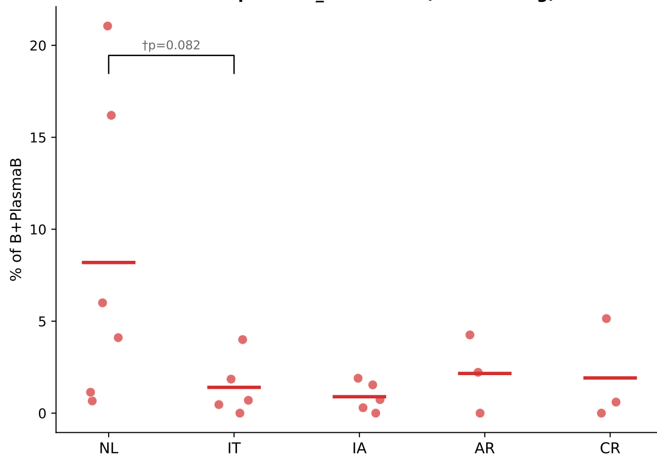
C. Liver plasmaB_c03-MKI67 (Proliferating)
