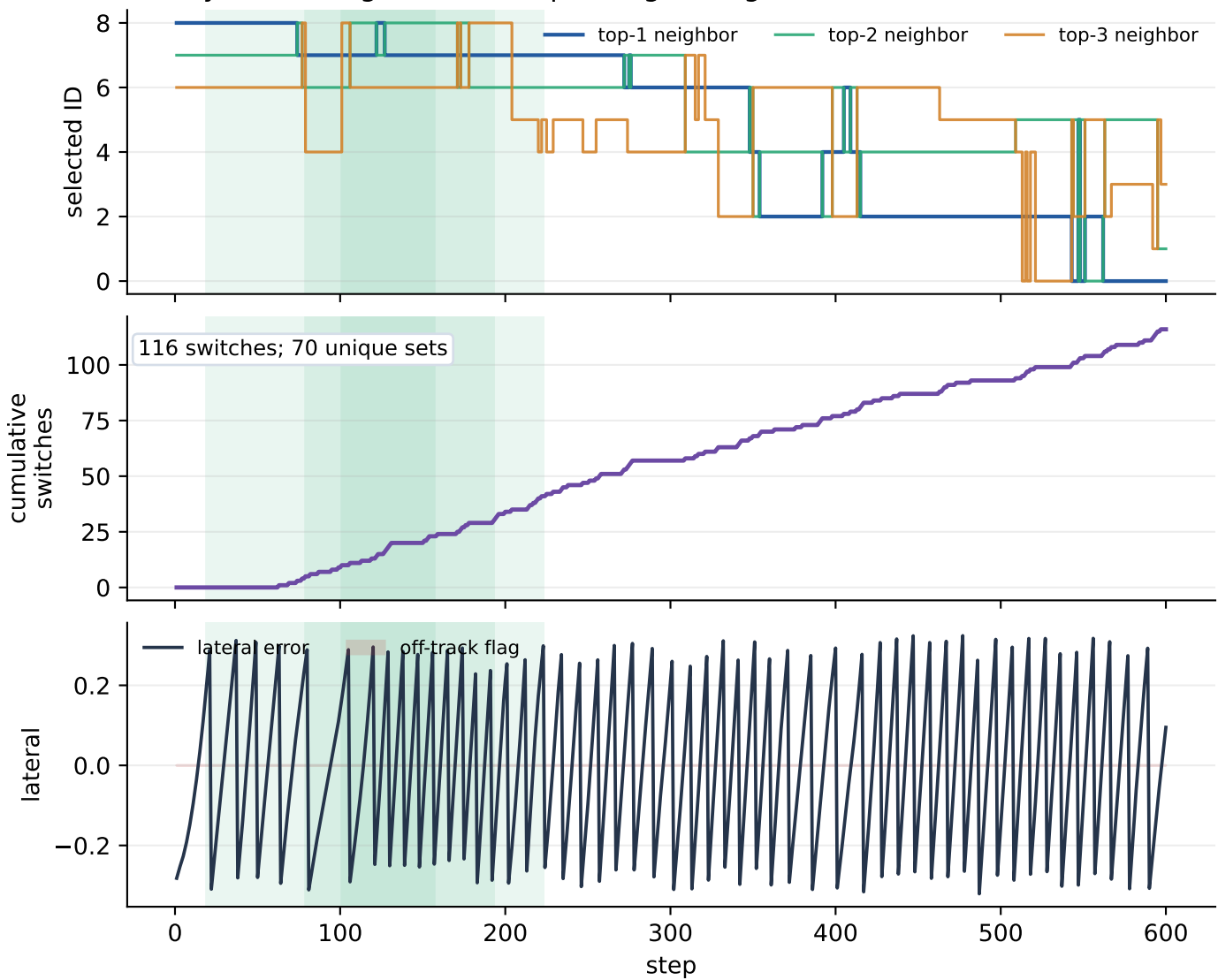
Dynamic-neighborhood repacking during a clean 10-vehicle overtake
