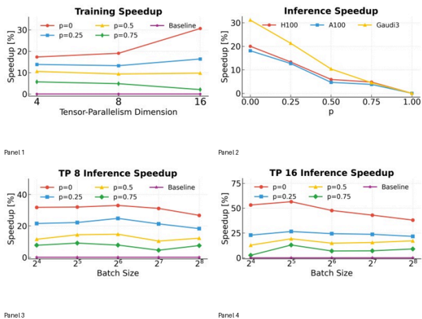
Figure 4: Speedup in training and inference for a Llama 7B model. Top Left Training speedup for varying values of p and tensor-parallel dimension. Top Right. Inference Time-To-First-Token (TTFT) speedup on different hardware, using batch-size 128. Bottom Left. Inference TTFT speedup using tensor-parallel 8 as a function of batch size, for different values of p . Bottom Right. Inference TTFT speedup using tensor-parallel 16 as a function of batch size, for different values of p .
