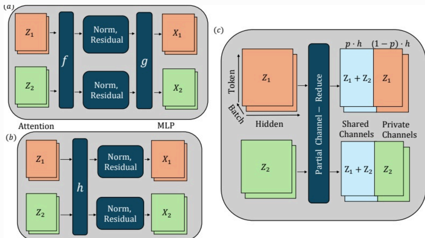
Figure 2: Partial synchronization and partial channel-reduce. (a) Vanilla transformers in current training frameworks. The operation f is an all-reduce in the forward pass and identity in the backward pass. The operation g is an all-reduce in the backward pass and identity in the forward pass. (b) With partial synchronization, h denotes the reduction operation in both the forward and the backward pass, since both must be done at the same location. Synchronization of the normalization function parameters is necessary. (c) Partial channel-reduce with parameter p over 2 devices.
