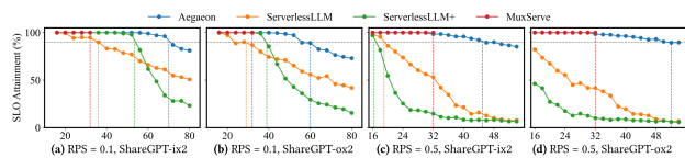
Figure 12. End-to-end SLO attainment under varying RPS with alternative datasets. x-axis: number of models.
