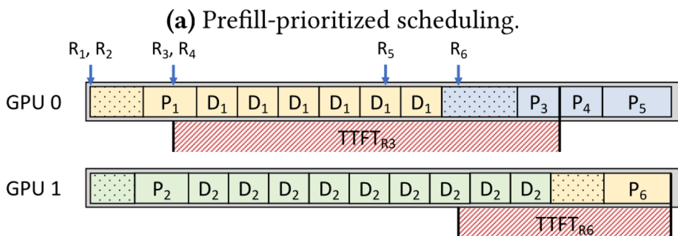
Figure 6. Exemplar token-level schedules on two GPUs. Prefill-first scheduling (a) and decoding-first scheduling (b) both lead to SLO violations. Disaggregated scheduling (c) separates prefill and decoding jobs to enable balanced token generation.
