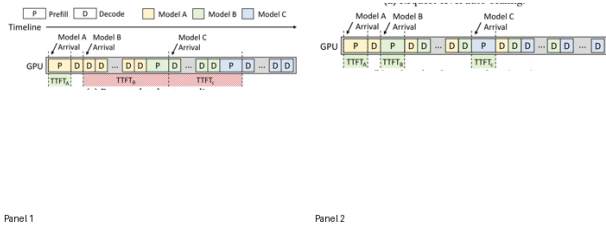
Figure 2. Different auto-scaling granularities for sharing one GPU instance between three models.
