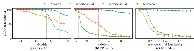
Figure 11. End-to-end SLO attainment under varying RPS with the ShareGPT dataset.
