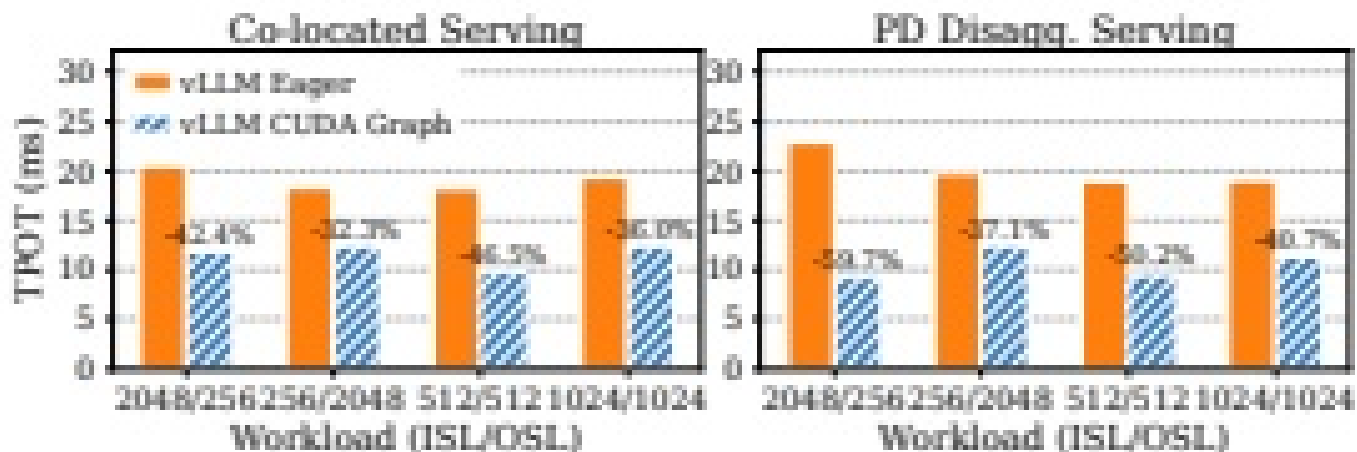
Figure 1. Measured vLLM TPOT with and without CUDA Graph under different workloads (64 requests per workload, mean ISL/OSL, tested on 8 \times \text{A800-SXM} GPUs). Left: co-location. Right: PDD. Percentages show reduction.
