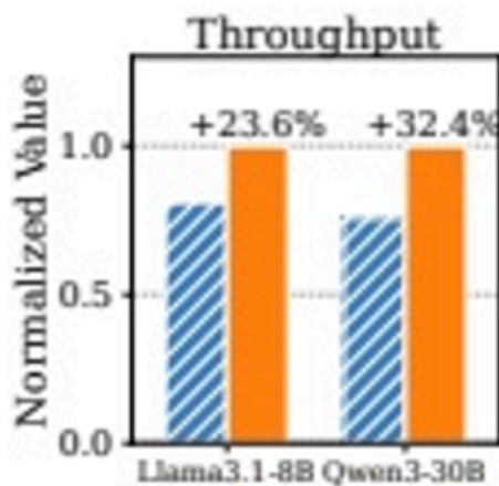
Figure 4. Fidelity gaps caused by simplified modeling. Left: Relying on coarse proxies (total token count) fails to capture batch heterogeneity, yielding coarse-grained performance estimates. Right: Analytical KV-cache modeling overestimates effective memory budget, leading to a cascade of errors from admission control to over-optimistic throughput projection.
