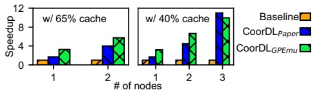
Figure 8: CoordDL's benefits with GPEMU (§3.4).
