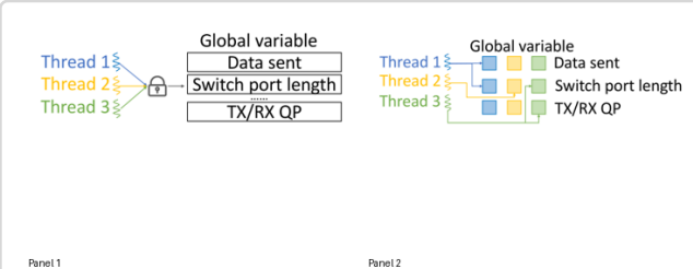
Figure 4: Multi-thread implementation and optimization in SimAI.
