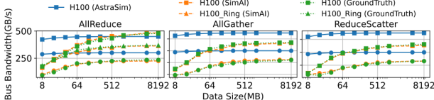
Figure 6: Bus bandwidths of intra-host collective communication operations vary with different message sizes and GPU types. Note that the performance is not related to the cluster scales.
