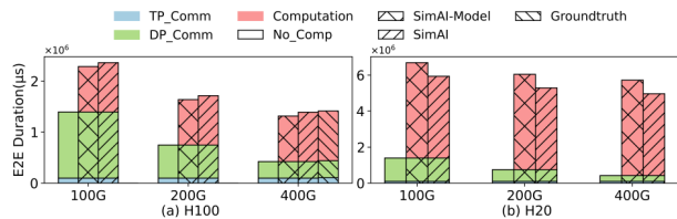
Figure 10: The iteration time of GPT-3 175B with different network bandwidths.
