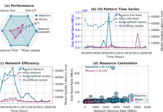
Figure 12: Network and I/O performance analysis comparing MLoRA with baseline. MLoRA achieves 89.5% reduction in network bandwidth and 60.2% reduction in disk I/O usage while significantly improving model update latency.
