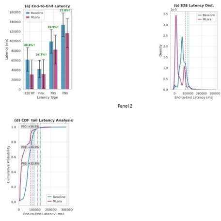
Figure 10: End-to-end performance comparison showing MLoRA achieves significant latency reduction compared to the baseline.
