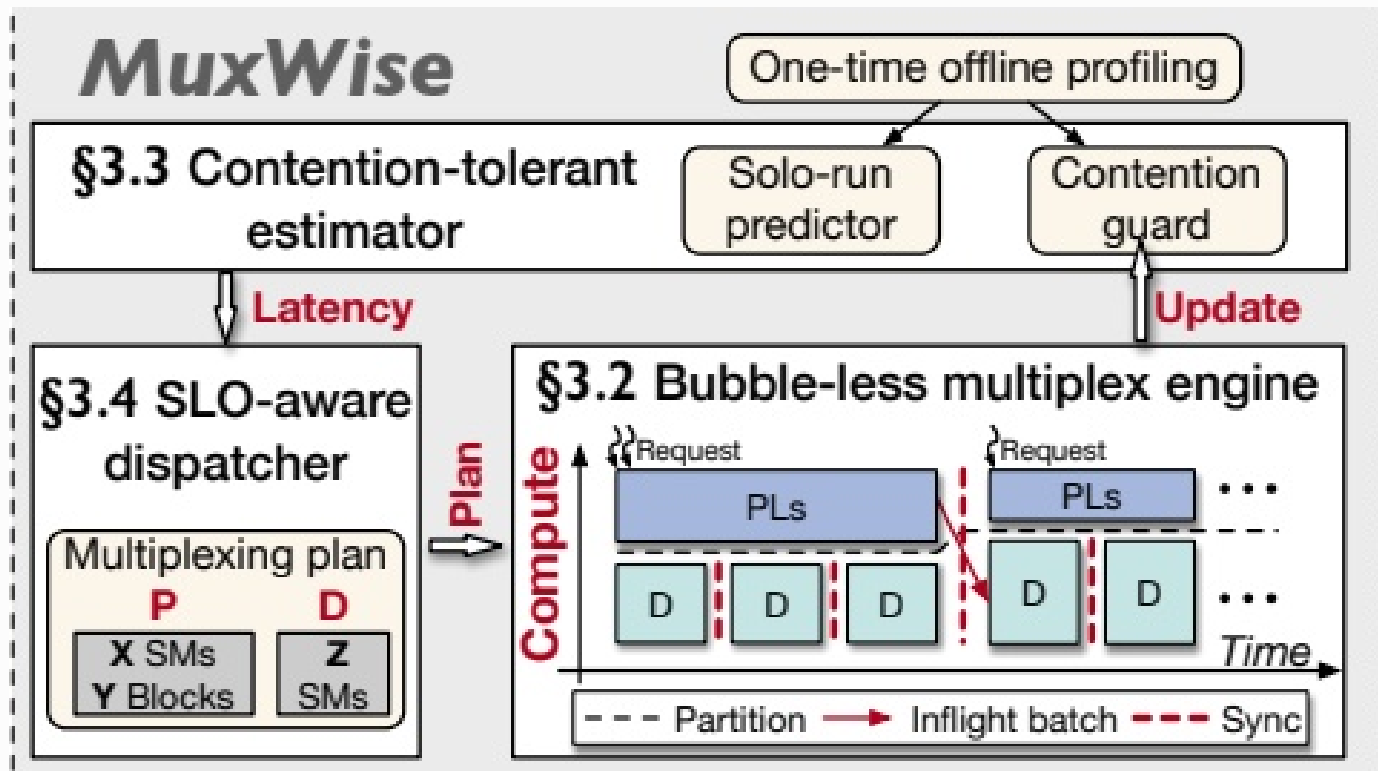
Figure 8. Architecture overview of MuxWise.
