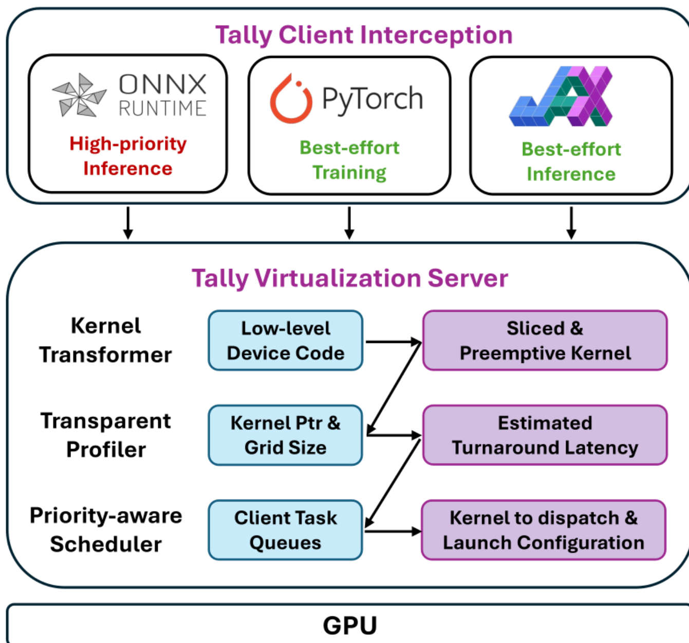
Figure 2. Tally architecture.
