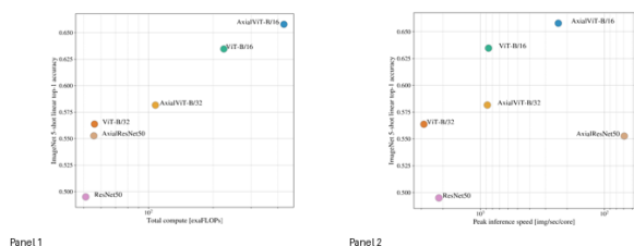
Figure 13: Performance of Axial-Attention based models, in terms of top-1 accuracy on ImageNet 5-shot linear, versus their speed in terms of number of FLOPs (left) and inference time (right).
