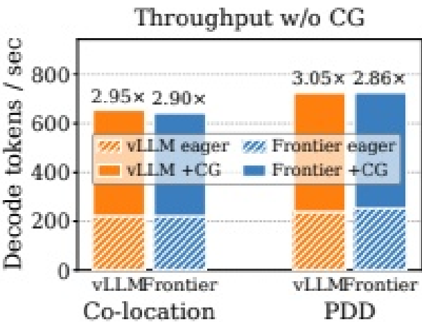
Figure 9. Decode throughput. +CG bars stack eager throughput with the CUDA Graph gain; top labels show total +CG/eager speedup. 来源：OCR 第 8 页。
