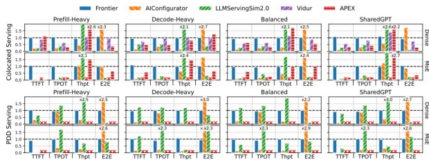
Figure 11. End-to-end fidelity on a 16-card H800 testbed for collocation and PDD across prefill-heavy, decode-heavy, balanced, and SharedGPT workloads. Panels report TFT, TPOT, throughput, and E2E makespan for both Llama3.1-8B (dense) and Qwen3-30B MoE; dashed bars indicate simulators that do not support the serving architecture or model family. All data are normalized against the ground truth (vLLM), represented by the black line ( y=1.0 ).
