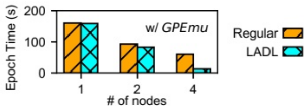
Figure 9: LADL's [80] benefits shown with GPEMU (3.4). 来源：OCR 第 9 页。
