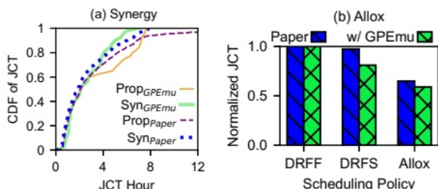
Figure 10: (a) Synergy [60] and (b) Allox's [54] JCT reduction with GPEMU. 来源：OCR 第 9 页。
