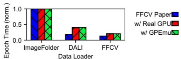
Figure 7: FFCV's [55] benefits shown with GPEMU (§3.3). 来源：OCR 第 8 页。
