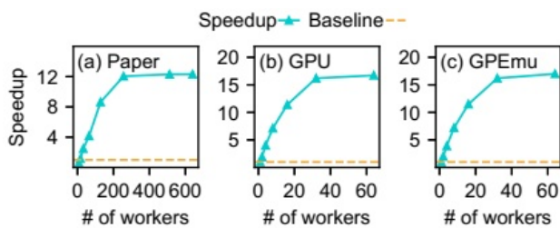
Figure 5: TF-DS [34] training speedup with GPEMU (§3.2). 来源：OCR 第 8 页。
