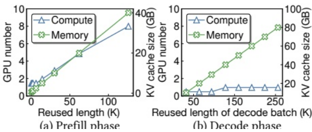
Figure 3. Required compute and memory for processing different phases under SLO constraints with varied reused context lengths. For prefill (a), the batch size is fixed at 1, the new context length is set to 2K, and TTFT is set to 400ms. For decode (b), the batch size is fixed at 32, and TBT is set to 100ms. These settings are commonly seen in online serving.
