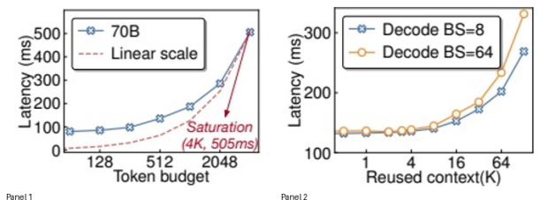
Figure 6. (a) Sweet spot of the token budget in chunk-prefill. The decode uses a fixed batch size of 32, with each request having a reused context length of 1K tokens. (b) Latencies with varied reused context of the fused prefill chunk in chunk-prefill. The token budget is fixed at 512, and the reused context length of decode phase is the same as in (a).
