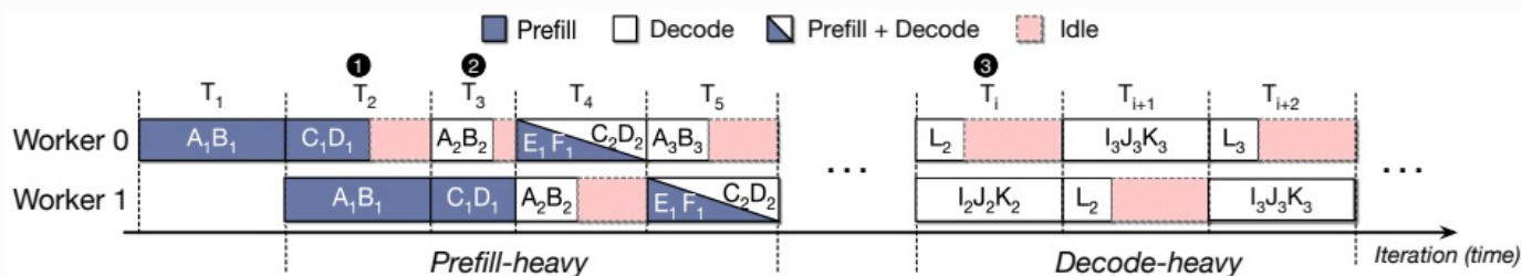
Figure 2: Three types of pipeline bubbles (The subscript indicates the iteration number.)
