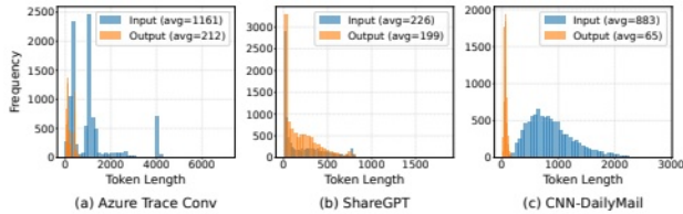
Figure 8: Input and output length distributions
