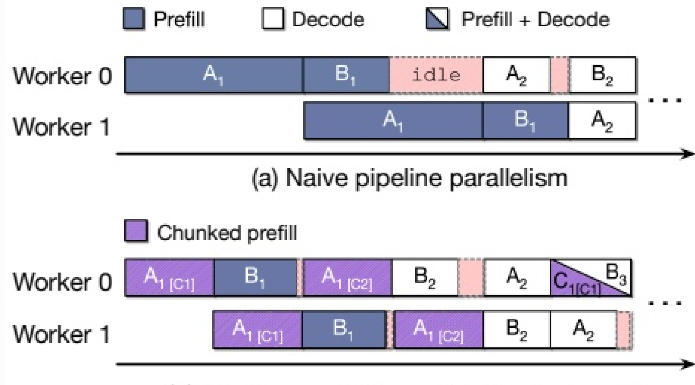
Figure 5: Reducing pipeline stalls from chunked-prefill [2]
