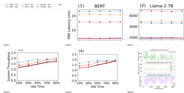
Figure 6. (a) Latency and throughput for high-priority BERT and Llama2-7B inference co-located with BERT, GPT-2, and Whisper training under Tally and TGS across different traffic loads. (b) Time-series visualization of user traffic, tail latency, and throughput over time for BERT inference co-located with BERT training across different GPU sharing systems.
