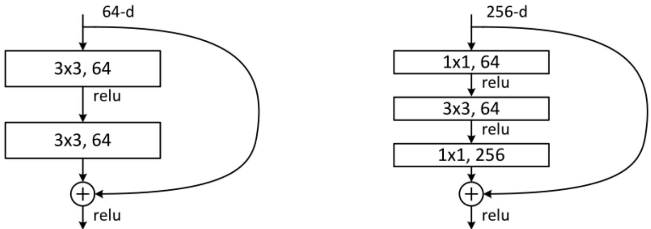
Figure 5. A deeper residual function for ImageNet. Left: a building block (on feature maps) as in Fig. 3 for ResNet-34. Right: a "bottleneck" building block for ResNet-50/101/152.
