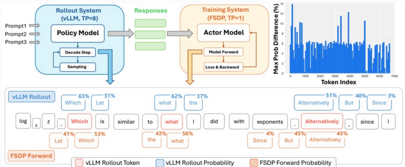
Figure 1. Illustration of probability discrepancies in RL training. Different frameworks and TP sizes produce noticeably probability gap for the same response, hindering stable and truly on-policy RL.
