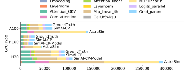
Figure 8: The execution time of the computation kernels of GPT-3 175B on different GPUs.
