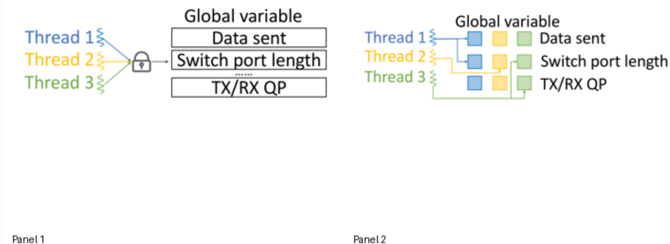
Figure 4: Multi-thread implementation and optimization in SimAI. 来源：OCR 第 8 页。
