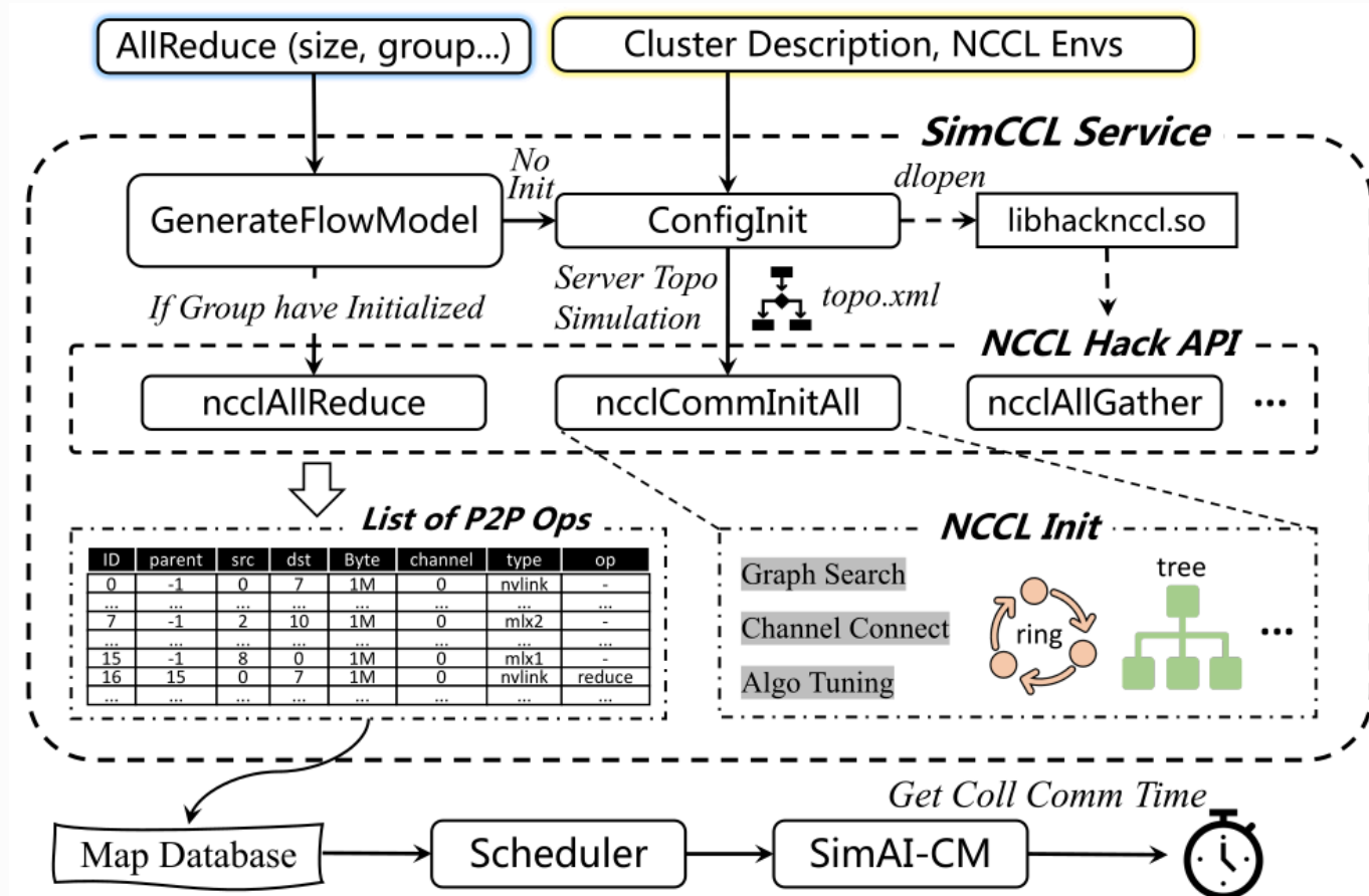
Figure 3: Illustration of how SimAI transforms a collective communication operation to a list of peer-to-peer communication operations. 来源：OCR 第 7 页。
