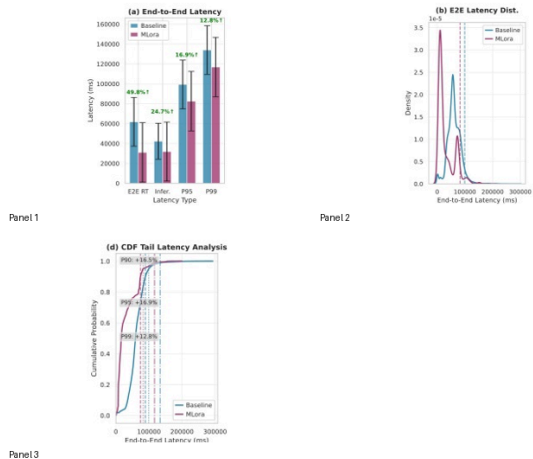
Figure 10: End-to-end performance comparison showing MLoRA achieves significant latency reduction compared to the baseline. 来源：OCR 第 11 页。
