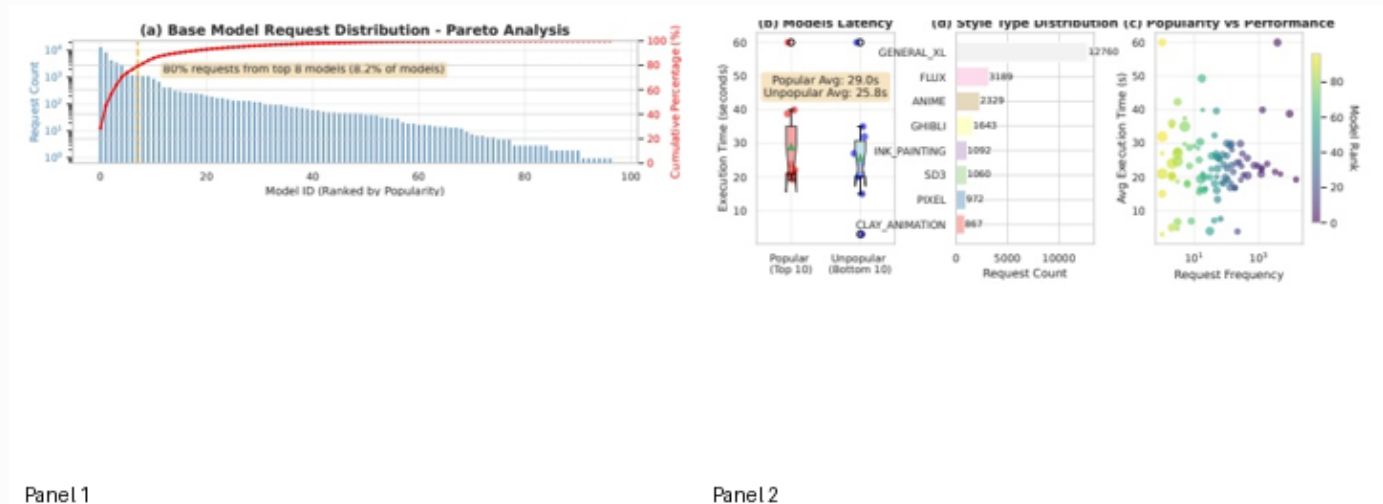
Figure 2: Base model request skewness analysis. The Gini coefficient of 0.876 indicates a highly skewed distribution, with the top 1 model accounting for 28.8% of requests. This highlights the significant concentration of requests on a few popular models, leading to resource allocation challenges.
