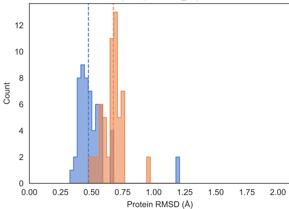
Scaffold 3 (ref: Mpro-x0107_0A)
