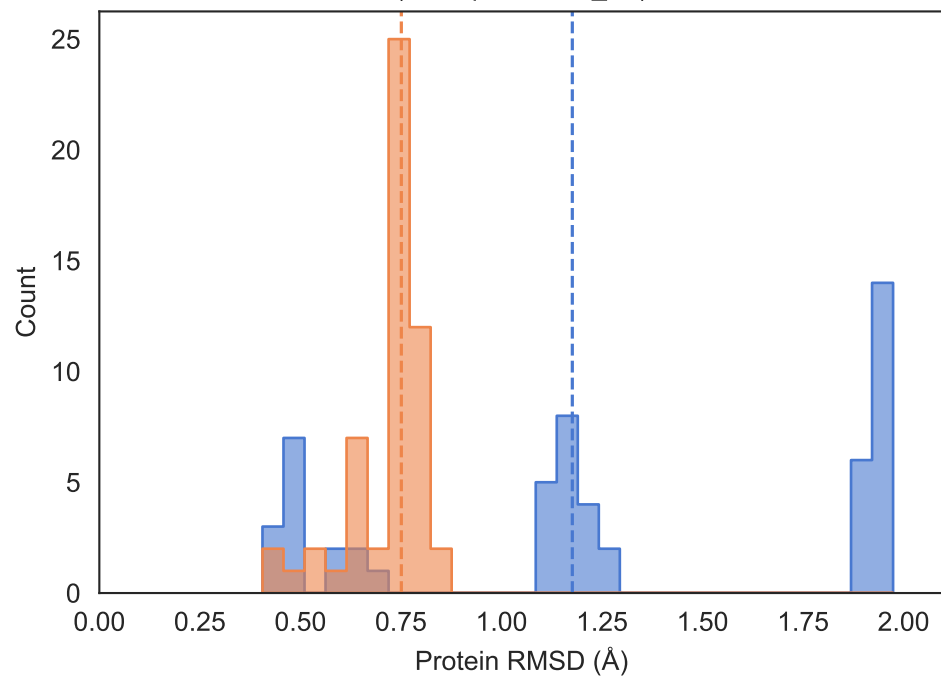
Scaffold 4 (ref: Mpro-P1835_0A)
