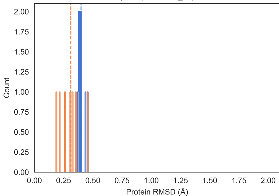
Scaffold 4 (ref: Mpro-P1835_0A)
