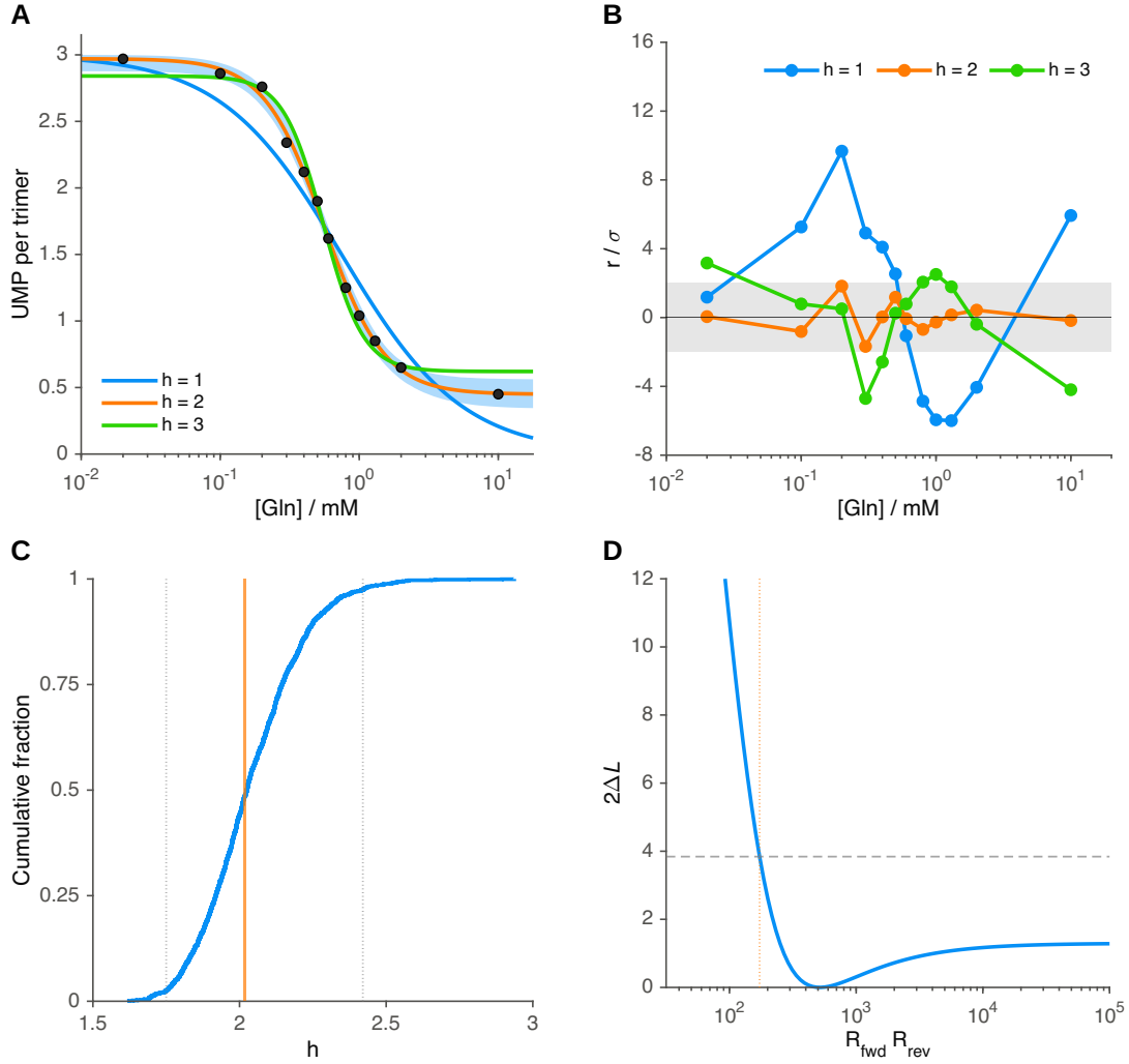
Figure S13: Information in the digitized first-layer titration. (A) Digitized coordinates and bounded fits with h=1 , 2, and 3. The fitted exponent, 2.018, nearly coincides with h=2 . Shading spans pointwise 2.5th–97.5th percentiles under coordinate perturbations. (B) Fixed-exponent residuals divided by the common h=2 residual scale, approximately 0.0407 UMP per trimer. (C) Fitted-exponent cumulative distribution from 2,000 coordinate perturbations; dotted lines mark the central 95% range. This is not an experimental replicate distribution. (D) Profile-likelihood loss for the regulatory swing. The horizontal criterion is 3.841 and its finite lower endpoint is approximately 173. The reciprocal-regulation interpretation is conditional on the plateau model.
