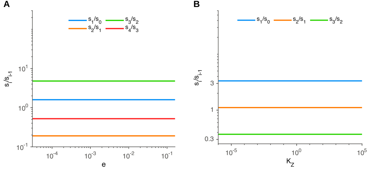
Figure S1: Numerical checks of the steady-state invariant. (A) Adjacent free-target ratios over a 5,278-fold enzyme sweep at fixed free effector in a four-site nonidentical ladder. (B) A three-site example with a reversible dead end swept over eleven decades at fixed total effector. The small ratio drift reflects the changed free effector; it is not a violation of the free-input identity. See S10 and the source parameter records.
