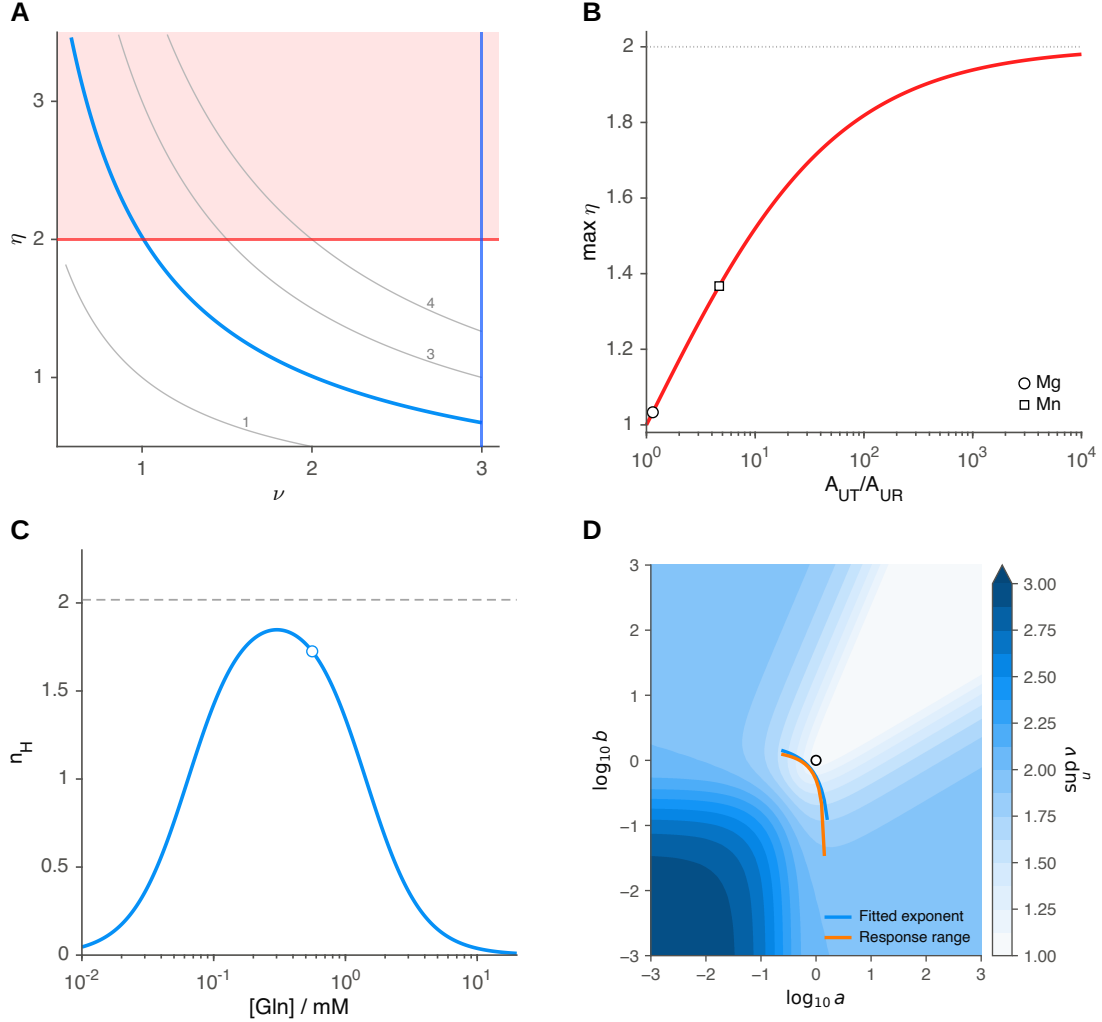
Figure S2: Local factorization and estimator-dependent ladder constraints. (A) Gray contours denote local products \nu \eta of 1, 3, and 4. The blue contour is a numerical reference at 2.018, not a measured local sensitivity. Red marks \eta=2 , the ceiling of the specified reciprocal switch, and dark blue marks the trimer bound \nu=3 . (B) Maximum switch elasticity for the reciprocal switch in S2 Appendix, D7 when A_{UT}/A_{UR} is at least one. Markers use the Mg and Mn kinetic-constant ratios discussed in the text. (C) Physical-occupancy local slope of the fitted first-layer curve, its fitted exponent of 2.018 (dashed), and midpoint local slope of 1.725 (circle). (D) Three-site ladder coefficients (1,3a,3b,1): distinct parameter loci reproduce coefficient ratio 1.11055 under fitted-exponent (blue) and response-range (orange) estimators. Color gives the maximum local ladder factor over input; the circle is the independent ladder. The loci are conditional calculations and show that the coefficient alone does not identify a unique ladder.
