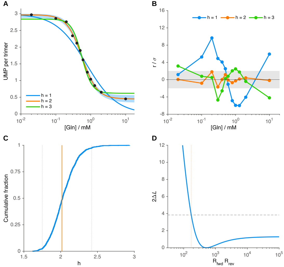
Figure S3: Information in the digitized first-layer titration. (A) Digitized coordinates and bounded fits with h=1 , 2, and 3. The fitted exponent, 2.018, nearly coincides with h=2 . Shading spans pointwise 2.5th–97.5th percentiles under coordinate perturbations. (B) Fixed-exponent residuals divided by the common h=2 residual scale, approximately 0.0407 UMP per trimer. (C) Fitted-exponent cumulative distribution from 2,000 coordinate perturbations; dotted lines mark the central 95% range. This is not an experimental replicate distribution. (D) Profile-likelihood loss for the regulatory swing. The horizontal criterion is 3.841 and its finite lower endpoint is approximately 173. The reciprocal-regulation interpretation is conditional on the plateau model.
