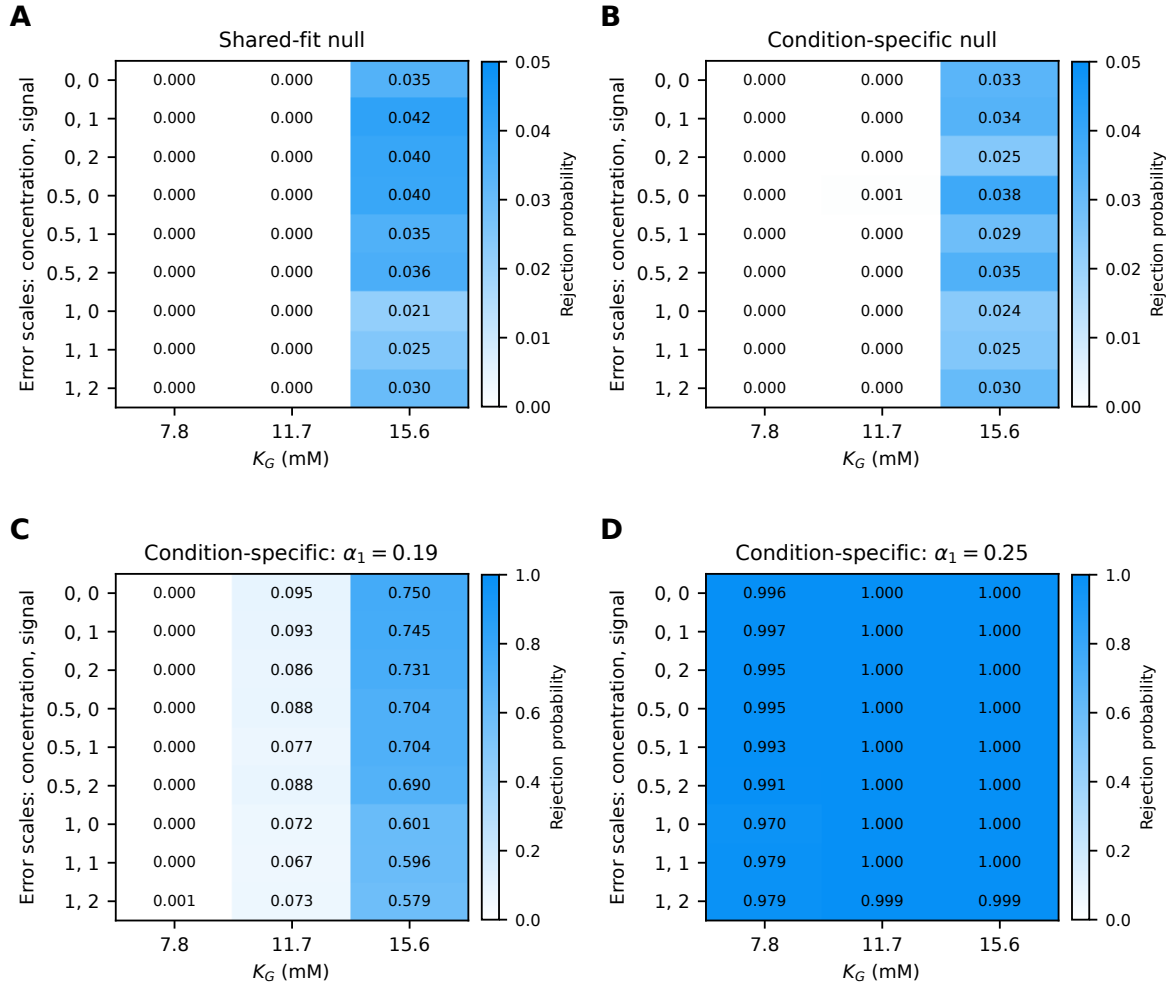
Figure S9: All audited nuisance cells for the null and two alternative effects. Each cell gives the rejection proportion from 2,000 independently evaluated trials after separate parametric calibration. Rows cross concentration-error scales c = 0, 0.5, 1 with signal-error scales s = 0, 1, 2 ; their physical error magnitudes are defined in S3 Appendix E5. (A–B) Shared and condition-specific fits under the \alpha_1 = 0.17 reference. (C–D) Condition-specific fits under \alpha_1 = 0.19 and 0.25 . Null panels use a 0–0.05 color scale; alternative panels use 0–1. Printed values are rounded to three decimal places. These are a discrete sensitivity grid, not an interpolated continuous performance guarantee.
