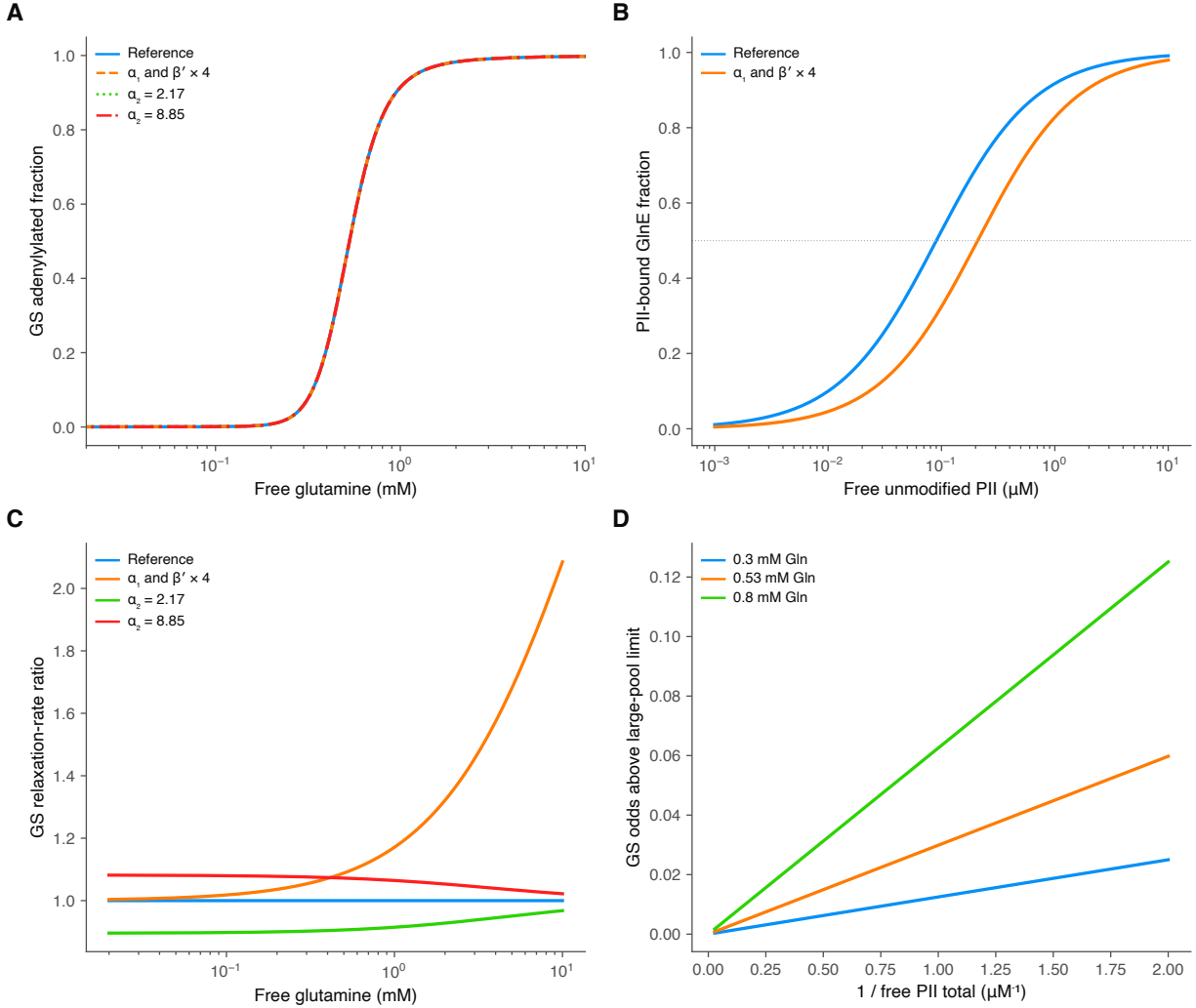
Figure S16: Binding and catalytic regulation in the published six-state GlnE topology. (A) Coupled GS steady-state curves are identical after a shared binding/catalysis transformation or a change in the PII–PII-UMP interaction parameter. One reference gain sets Y = 0.5 at 0.53 mM glutamine and T = 5 \mu\text{M} ; it is unchanged in every variant. (B) PII-binding isotherms at fixed G = 10 mM and U = 0.3 \mu\text{M} distinguish binding from catalytic synergy. (C) Reduced GS relaxation rates at separately controlled P = 1 \mu\text{M} and U = 0.3 \mu\text{M} differ along a glutamine titration. These are not the coupled inputs in A. (D) The PII-independent route gives a drive affine in inverse free-target total at fixed glutamine and modification fraction. Its analytic large-pool limit is subtracted to display the concentration-dependent term. Lines are predictions, not additional observations. S21 separates source-reported fitted constants from chosen parameters and states the rapid-binding and independent-GS assumptions.
