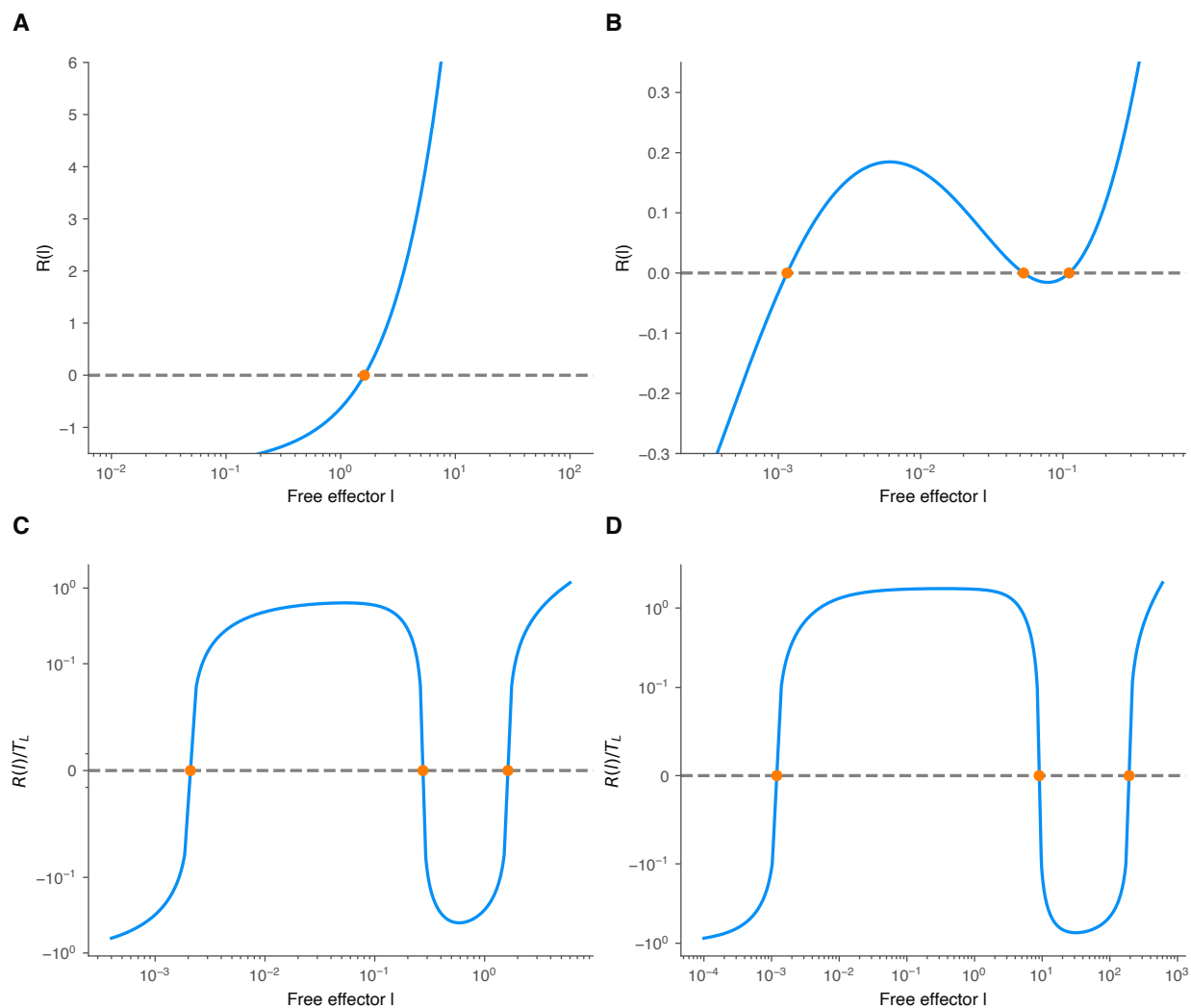
Figure S5: Uniqueness conditions and verified multistationarity. (A) Corrected independent-site kinetic example satisfying both conditions. (B) Original four-site example with catalytic-ratio spread 2.89: three positive states, but both conditions are violated. (C) Constant catalytic ratios with condition (ii) violated. (D) An exact binomial ladder satisfying condition (ii) globally, with condition (i) violated and three physical states. Panels C and D use residual divided by total effector with symmetric logarithmic vertical axes. Markers are refined roots, not neighboring grid points. S11 and S1 Data specify all parameters, positivity checks, and the exact root count for D. Stability is not encoded by the marker style.
