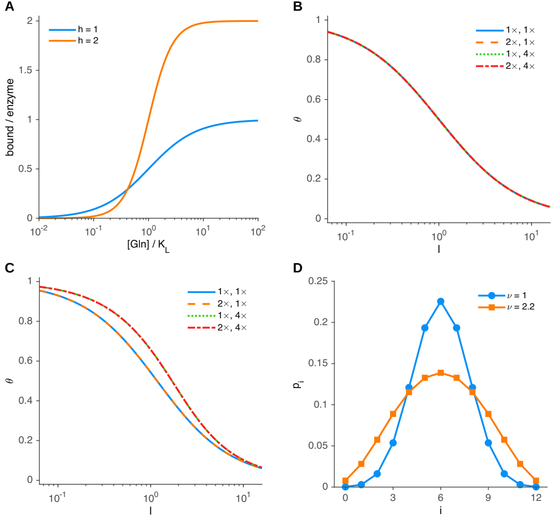
Figure S8: Measurements that discriminate unresolved mechanisms. (A) Illustrative one-ligand and concerted two-ligand binding laws, expressed as ligands per enzyme. Activity measurements must accompany occupancy to identify productive states. (B) Illustrative minimal-model total-target responses at two enzyme and two target levels. Parameters are n=3 , A=1 , \hat{B}=\hat{G}=0.4 , \hat{K}=1 , baseline T_E=0.0001 and T_S=1 in consistent concentration units; the four curves nearly coincide because the enzyme pool is dilute. (C) An illustrative active target-bridging extension with one modification site and relation s_1=s_0/(1-0.35s_0) , with total free target 1 or 4. Target levels separate; enzyme levels coincide in this reduced construction. These examples are not fits to the measured titration. (D) Twelve-site distributions with the same mean modification but \nu=1 or \nu=2.2 , generated by exponential reweighting of binomial states as specified in S1 Appendix. These distributions are not fits to glutamine synthetase.
