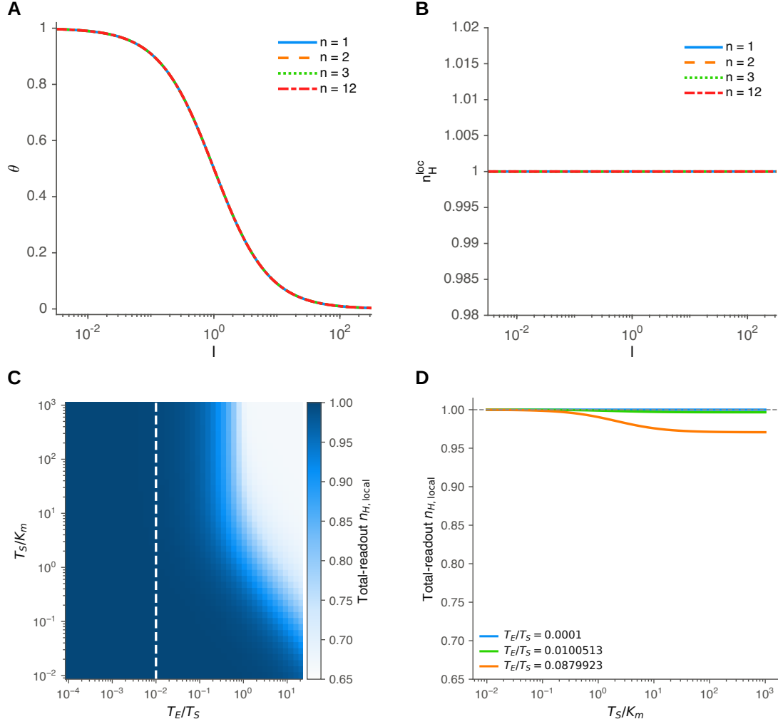
Figure S1: Independent-site invariance and the experimentally accessible readout. (A) Free-target mean modified fractions for n=1, 2, 3 , and 12 identical independent sites coincide, with dimensionless input and unit midpoint. (B) Their local coefficients equal one throughout. (C) Local coefficient of the total-target readout at half-response across enzyme-to-target ratio and target saturation in the specified three-site model; the dashed line marks T_E/T_S=0.01 . (D) Representative slices. For T_E/T_S at most 0.01 the coefficient remains at least 0.99745 across the plotted saturation range. Panels C and D are numerical calculations for the stated model; the exact invariant in A and B concerns free target.
