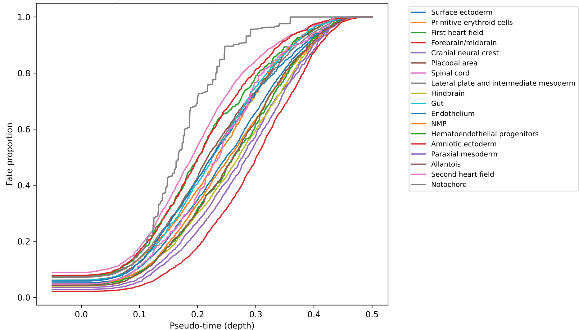
Average Fate Vector Components vs. Pseudo-time
