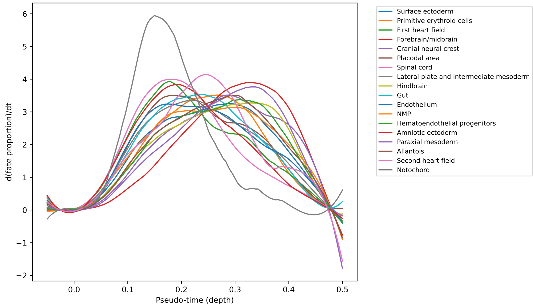
Fate Commitment Rate ( dv/dt ) vs. Pseudo-time
