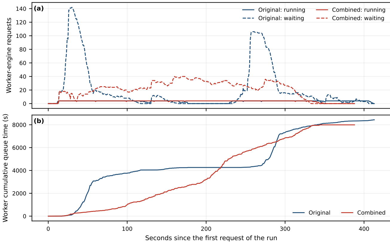
Concurrency 100, round 4: worker engine (tool-call formation and synthesis)
