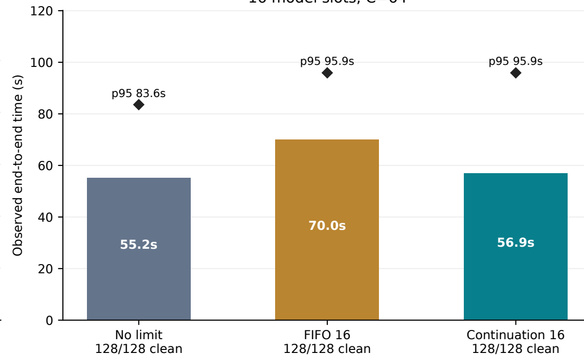
16 model slots, C=64
