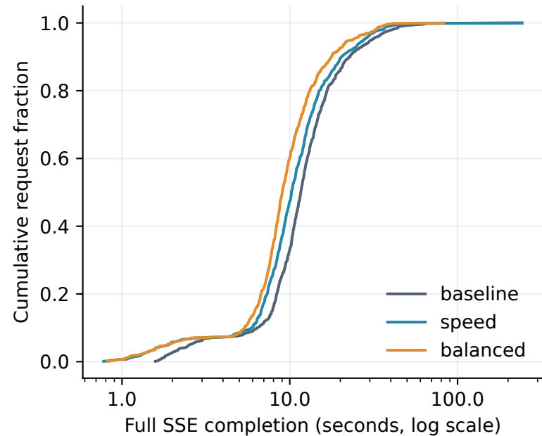
A End-to-end latency
