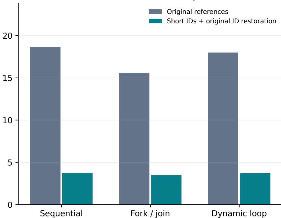
Mean workflow latency (s)
