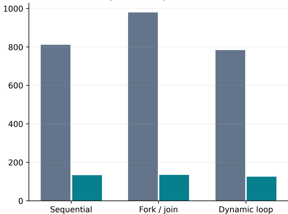
Output tokens per workflow
